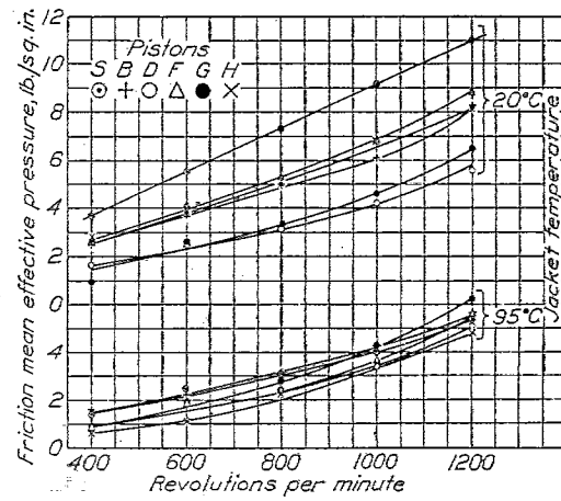
FIG. 26.—Pistons without rings; cylinder pressure nearly constant. ("No pumping loss")
