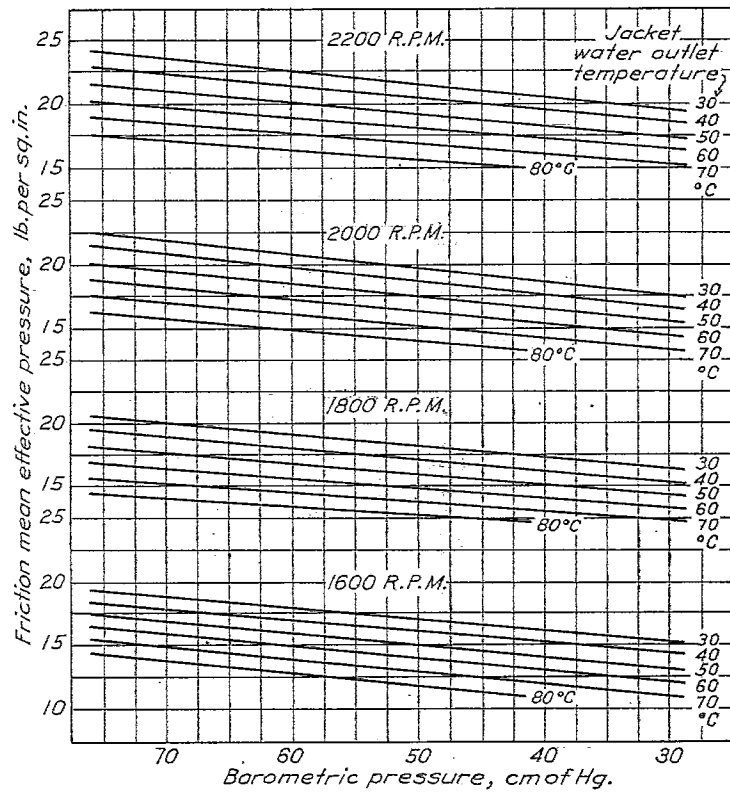
Fig. 5.—Compression ratio, 5.3. Engine C: 12 cylinders; bore, 4.5 inches; stroke, 6 inches
