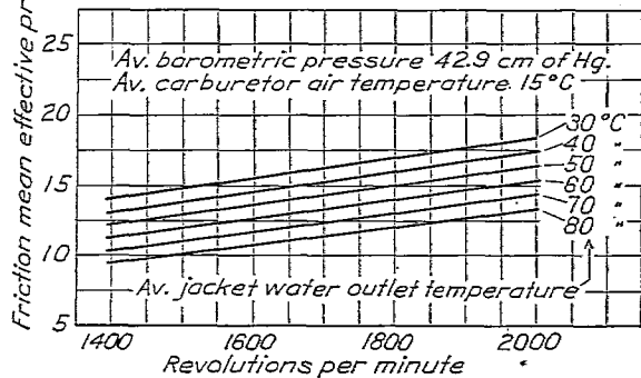
FIG. 8.—Engine A: 8 cylinders; bore, 5.51 inches; stroke, 5.91 inches; compression ratio, 6.5
