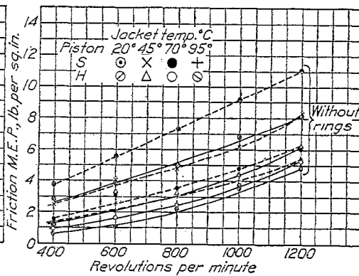
FIG. 24.—Pistons S and H: Friction mean effective pressure versus revolutions per minute; cylinder pressure nearly constant. ("No pumping loss")
